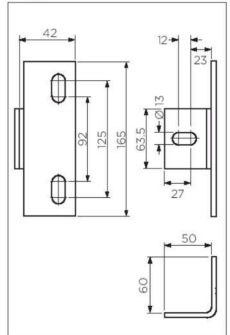
xxxxx6: Galvanized steel T metal bracket
